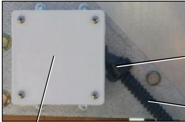
Rear discharge switch conduit at rear left gusset.
